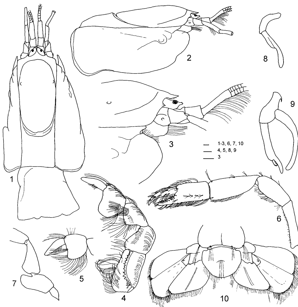
Figs. 1–10. Neocallichirus vigilax , RMNH D1481, female holotype of Callianassa vigilax DE MAN, 1916 (tl 85 cl 22): 1, carapace and first abdominal somite in dorsal view; 2, carapace in lateral view; 3, front in lateral view; 4, right third maxilliped, mesial view; 5, left third maxilliped, propodus and dactylus, lateral view; 6, minor cheliped, lateral view; 7, third pereopod, distal articles in lateral view (setae omitted); 8, right first pleopod, posterior view (setae omitted); 9, right second pleopod, posterior view (setae omitted); 10, tailfan. Scale is 1 mm.
