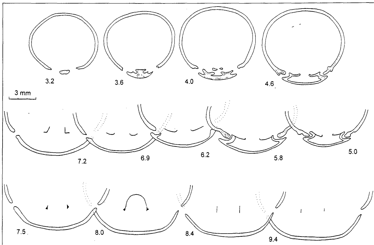
Text-Fig. 11. Lobothis delta (NEUMAYER). Eiberg, coll. PIW. Transverse sections through the specimen 26.4 mm long. Magnified.
