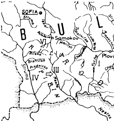
Fig. 1 Mesta river, Southwest Bulgaria
