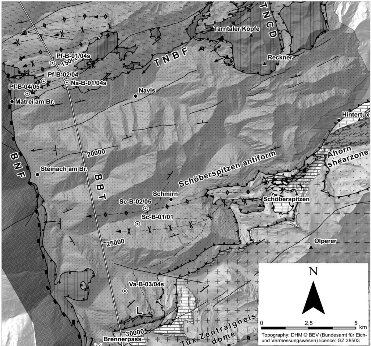
Strain partitioning on major fault zones in the northwestern Tauern Window – insights from the investigations to the Brenner Base Tunnel
